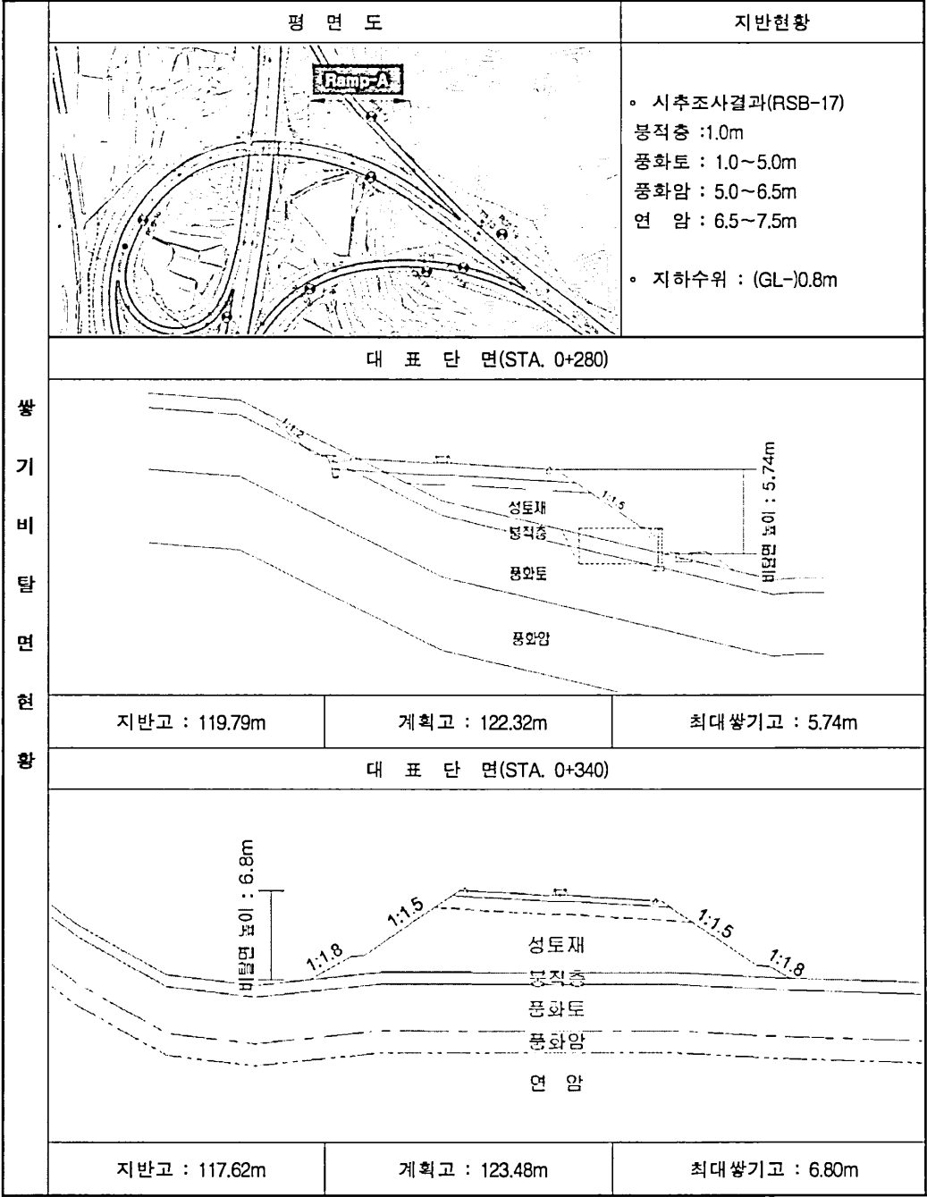
(19) Ramp - A (STA. 0+250~0+370, L=120.0m)
